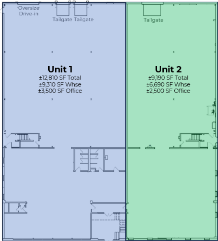
1st Floor
