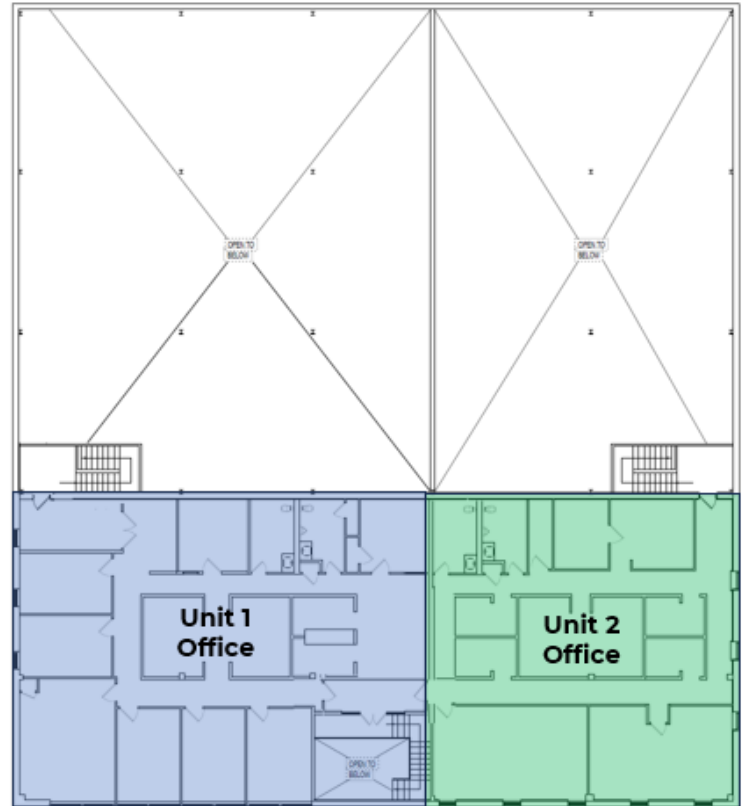
2nd Floor
